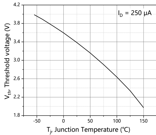
Figure 8. Threshold voltage
